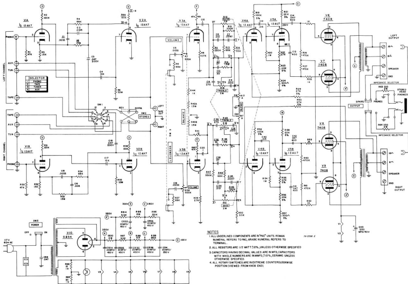
FIGURE 5 - AP30 SCHEMATIC DIAGRAM
